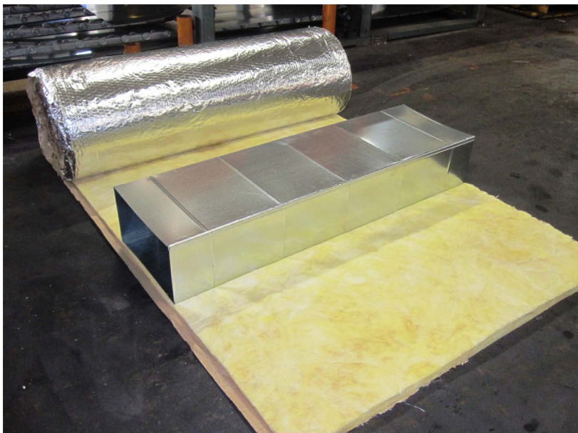
WideWrap™ is designed to work perfectly with 5' duct sections, saving labor and materials while resulting in cleaner-looking installs
